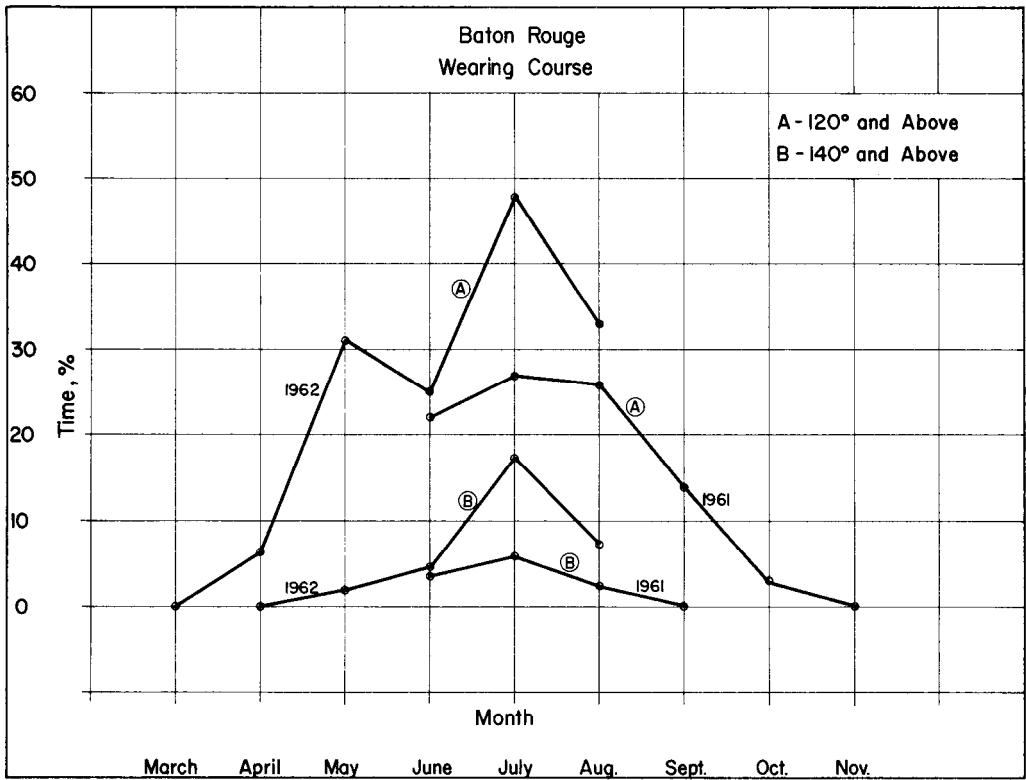
Figure 5 - Illustration of the Monthly Per Cent of Time Above 120°F and 140°F for the Wearing Course in the Baton Rouge Area.
